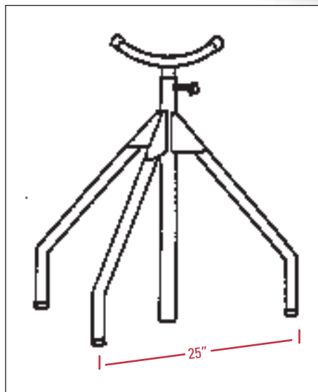
DEPLOYED
